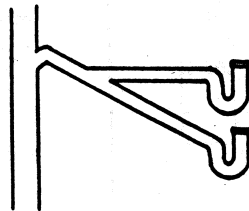
TWO TRAPS ON SAME ARM
