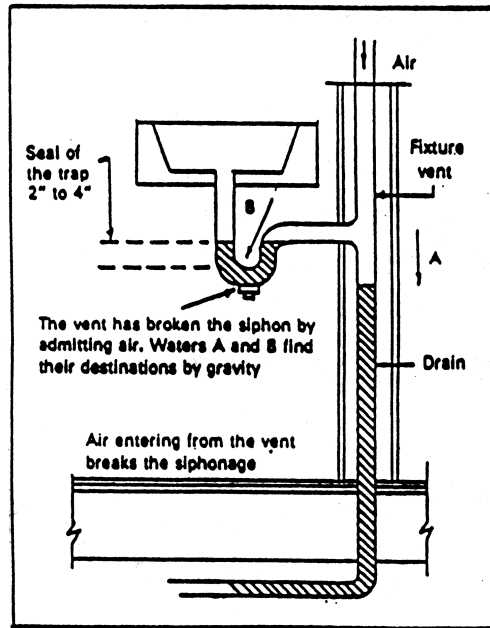
FIGURE 2202.2.1B — Example of Vented Trap
