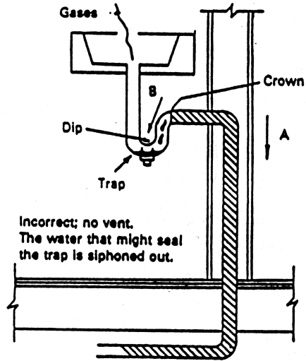
FIGURE 2202.2.1A — Example "S" Trap
