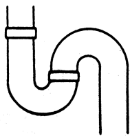
FULL S-TRAP
